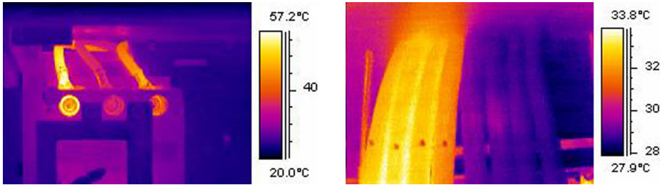
Figure 28.14 Examples of infrared images of load variations
