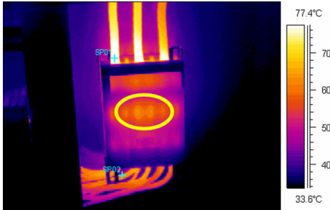
Figure 28.4 A hidden hot spot inside a box
