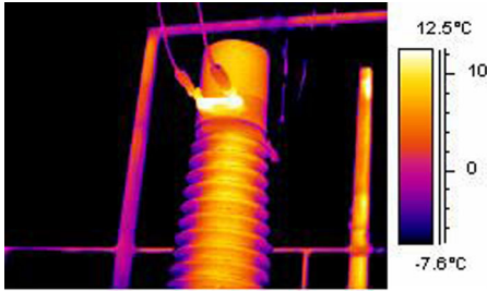
Figure 28.12 An infrared image of a circuit breaker
