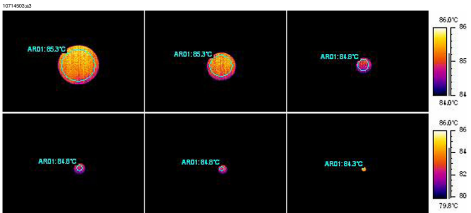
Figure 28.19 Temperature readings from a blackbody at +85°C (+185°F) at increasing distances
