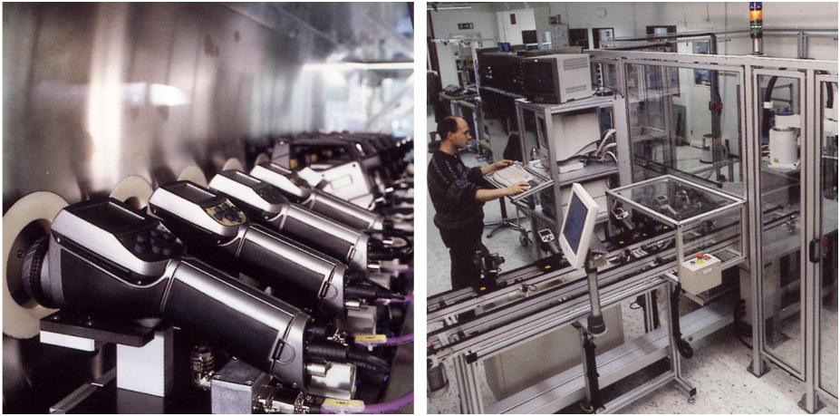
Figure 29.4 LEFT: Testing of infrared cameras in the climatic chamber; RIGHT: Robot used for camera testing and calibration
