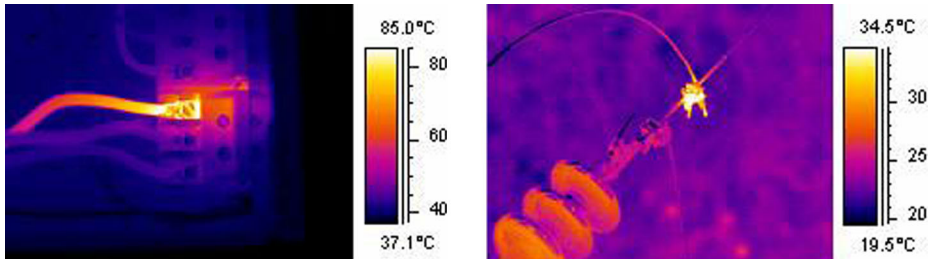
Figure 28.16 LEFT: An infrared image showing bad contact due to a loose bolt; RIGHT: A loose outdoor connection, exposed to the wind cooling effect.
