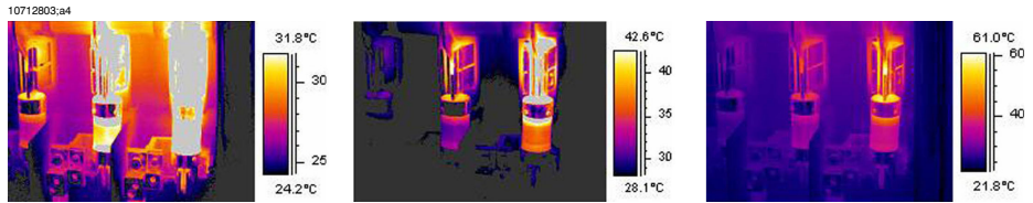
Figure 28.2 Temperature variations in a fusebox
