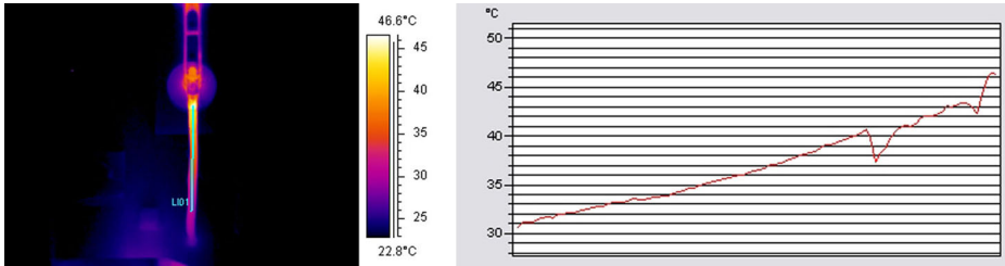
Figure 28.7 A profile (line) in an infrared image and a graph displaying the increasing temperature
