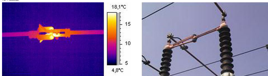
Figure 28.17 Overheating in a circuit breaker
