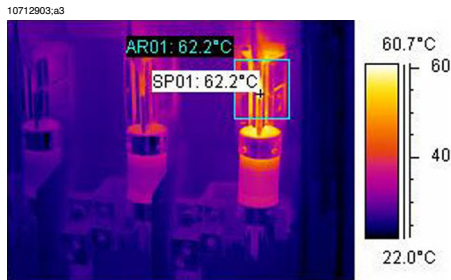
Figure 28.3 An infrared image of a fusebox where the maximum temperature is displayed
