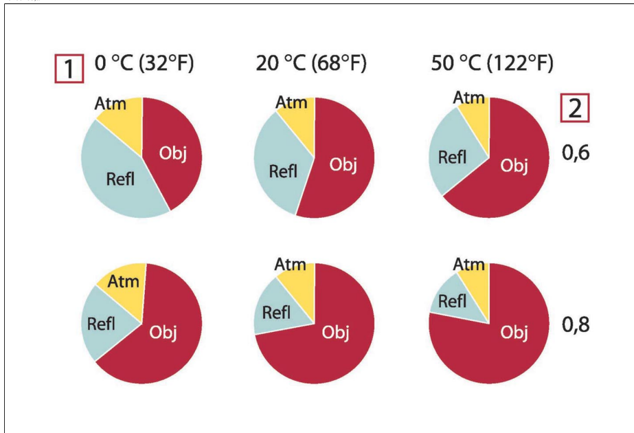
Figure 37.4 Relative magnitudes of radiation sources under varying measurement conditions (LW camera). 1: Object temperature; 2: Emittance; Obj: Object radiation; Refl: Reflected radiation; Atm: atmosphere radiation. Fixed parameters: \tau = 0.88 ; T_{refl} = 20^{\circ}\text{C} (+68°F); T_{atm} = 20^{\circ}\text{C} (+68°F).
