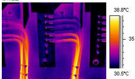
Figure 31.15 An infrared image of bundled cables
