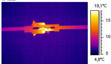
Figure 31.17 Overheating in a circuit breaker
