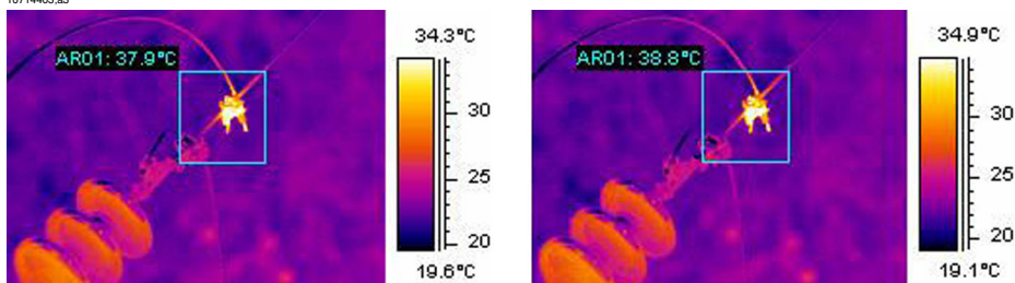
Figure 31.18 LEFT: Incorrect distance setting; RIGHT: Correct distance setting
