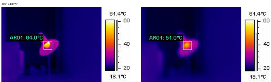
Figure 31.5 LEFT: A hot spot in focus; RIGHT: A hot spot out of focus
