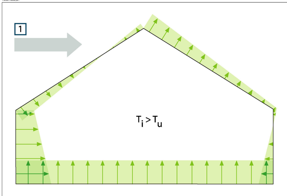
Figure 30.3 Distribution of resultant pressures on a building's enclosing surfaces depending on wind effects, ventilation and internal/external temperature difference. 1: Wind direction; T_u : Thermodynamic air temperature outdoors in K; T_i : Thermodynamic air temperature indoors in K.
