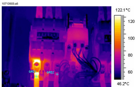
Figure 31.9 An infrared image of indoor electrical equipment (2).
