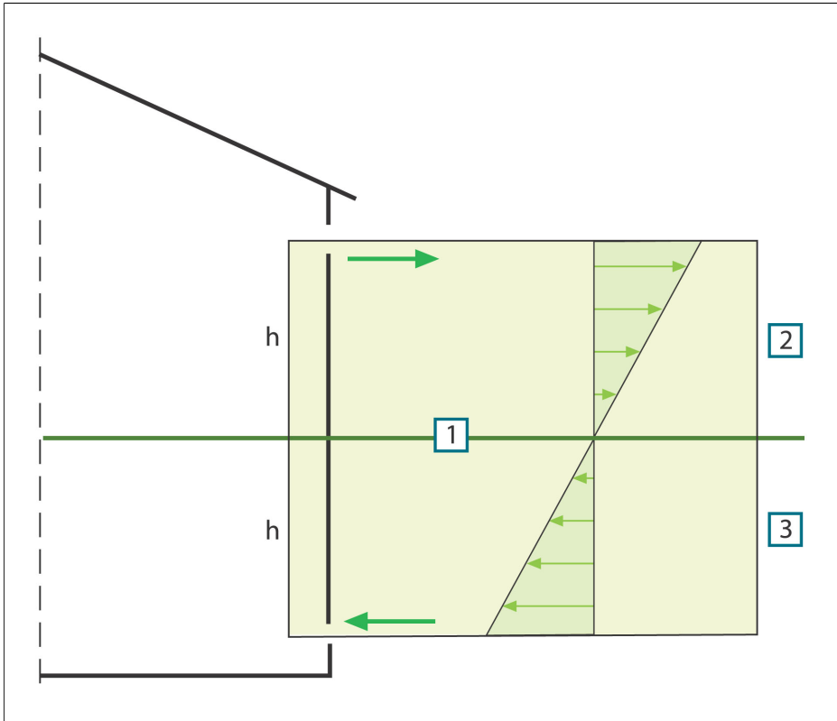
Figure 30.5 Distribution of pressures on a building with two openings and where the external temperature is lower than the internal temperature. 1: Neutral zone; 2: Positive pressure; 3: Negative pressure; h : Distance from the neutral zone in meters.
