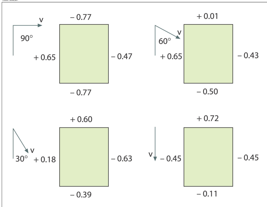
Figure 30.4 Stress concentration factor (C) distributions for various wind directions and wind velocities (v) relative to a building.
