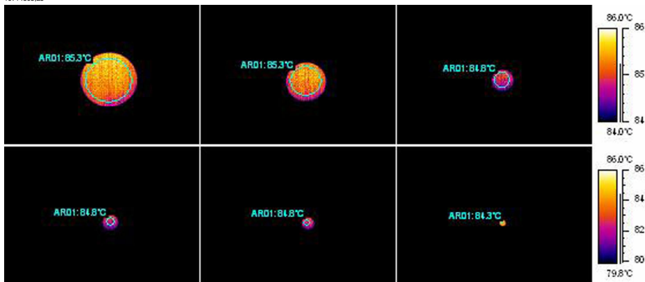
Figure 31.19 Temperature readings from a blackbody at +85°C (+185°F) at increasing distances
