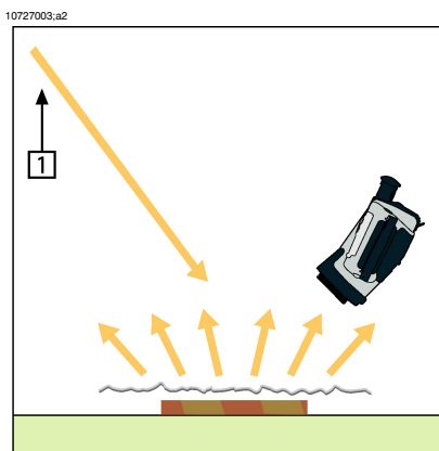
Figure 34.4 Measuring the apparent temperature of the aluminum foil
