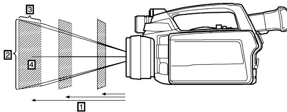
Figure 26.2 Relationship between field of view and distance. 1: Distance to target; 2: VFOV = vertical field of view; 3: HFOV = horizontal field of view; 4: IFOV = instantaneous field of view (size of one detector element).
