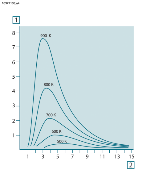
Figure 36.4 Blackbody spectral radiant emittance according to Planck's law, plotted for various absolute temperatures. 1: Spectral radiant emittance (W/cm 2 × 10 3 (μm)); 2: Wavelength (μm)
