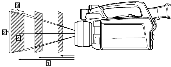
Figure 26.3 Relationship between field of view and distance. 1: Distance to target; 2: VFOV = vertical field of view; 3: HFOV = horizontal field of view; 4: IIFOV = instantaneous field of view (size of one detector element).
