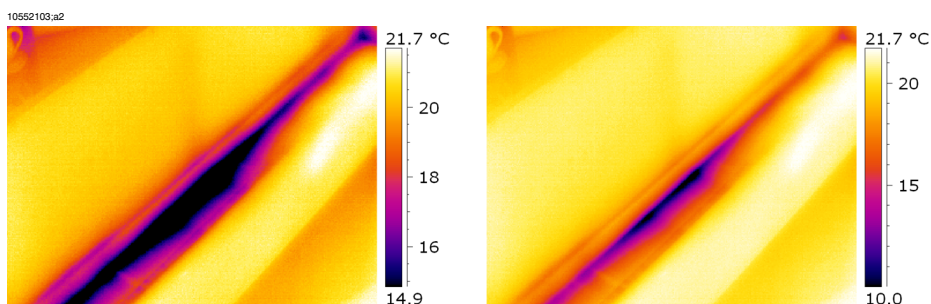
Figure 30.1 LEFT: A thermally untuned infrared image; RIGHT: A thermally tuned infrared image, after having changed level and span.
