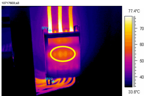
Figure 31.4 A hidden hot spot inside a box
