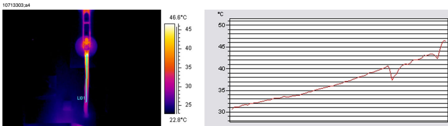
Figure 31.7 A profile (line) in an infrared image and a graph displaying the increasing temperature
